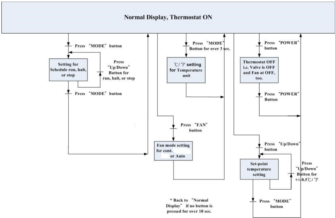
Fig. 2 User Mode operation sequence
